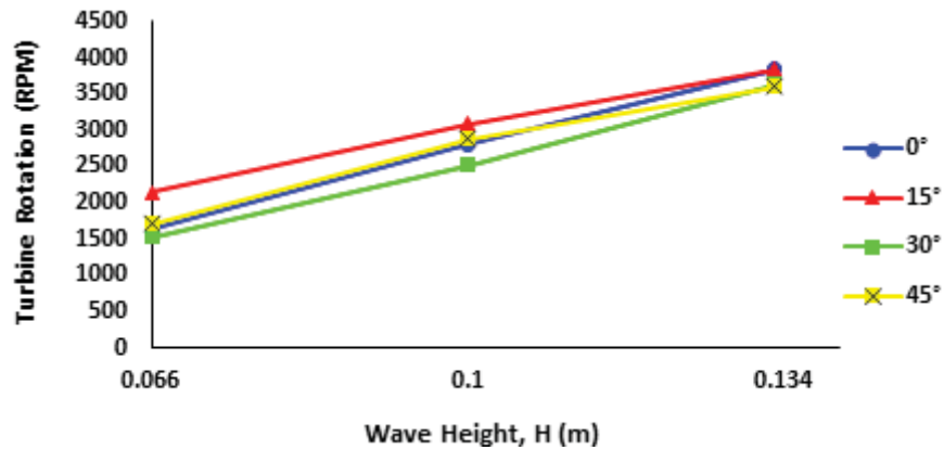
FIGURE 4. Turbine rotation vs wave height
