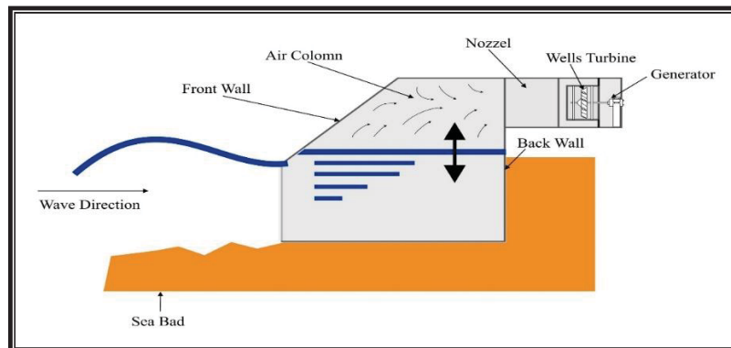
FIGURE 1. Schematic of OWC - Side view [2]
