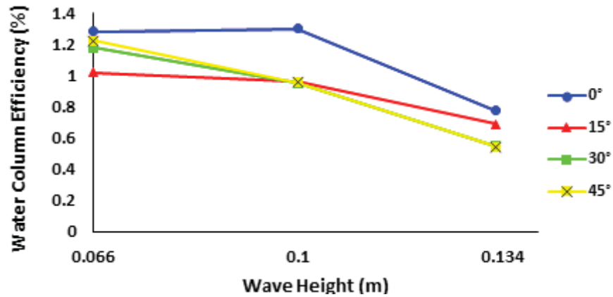
FIGURE 7. Water column efficiency vs wave height
