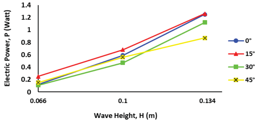
FIGURE 6. Electric power vs wave height
