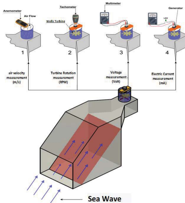
FIGURE 2. Variable measurement of testing experiment
