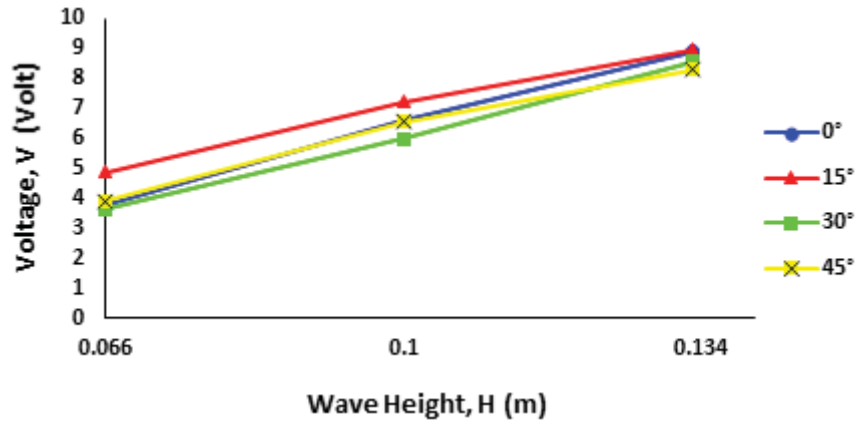
FIGURE 5. Electric voltage vs wave height
