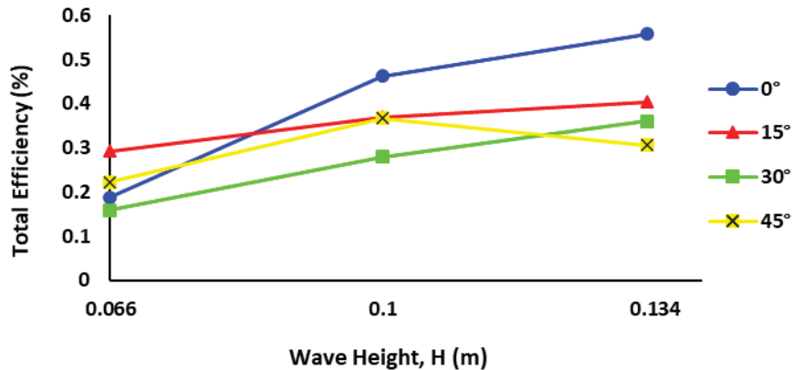
FIGURE 8. Total efficiency vs wave height
