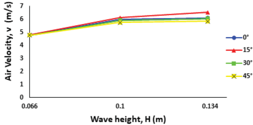
FIGURE 3. Air velocity vs wave height variation
